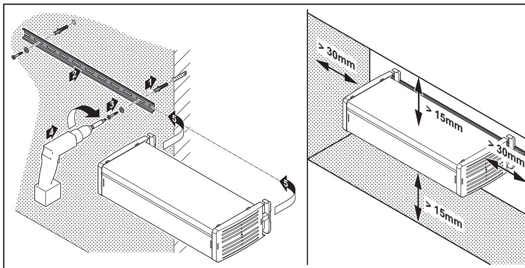
Charger with optional wall bracket (DIN rail TS 35, EN 50022)
